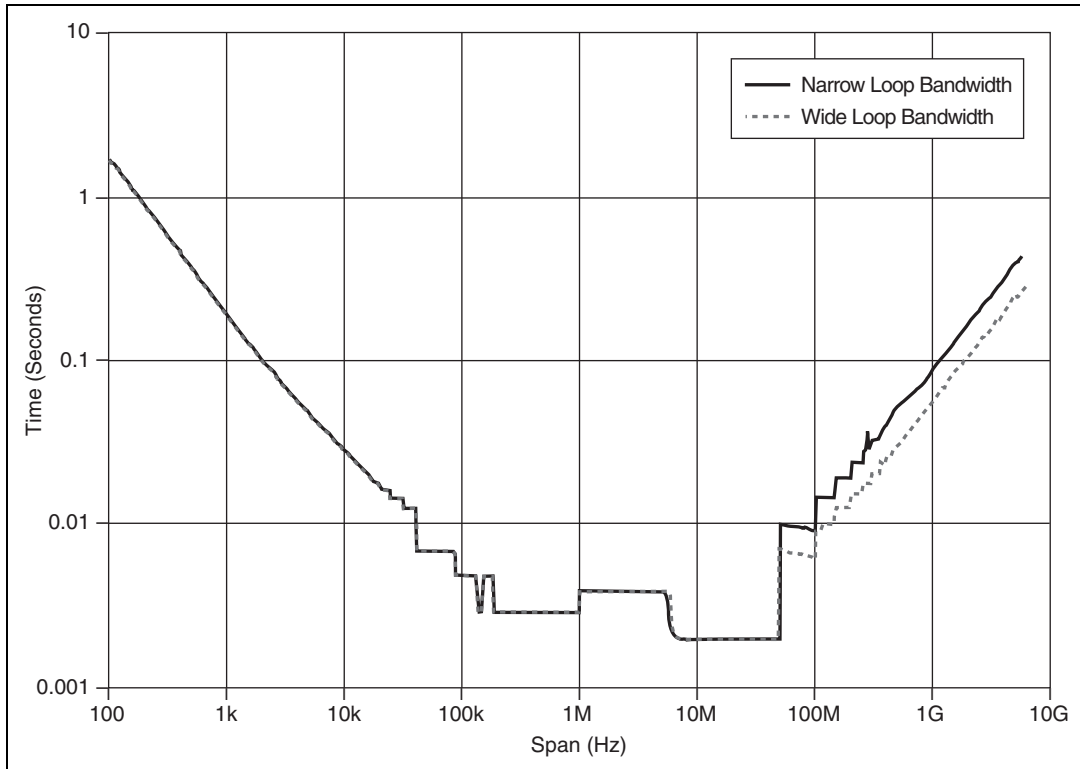
Figure 6. NI 5663E Measurement Time
