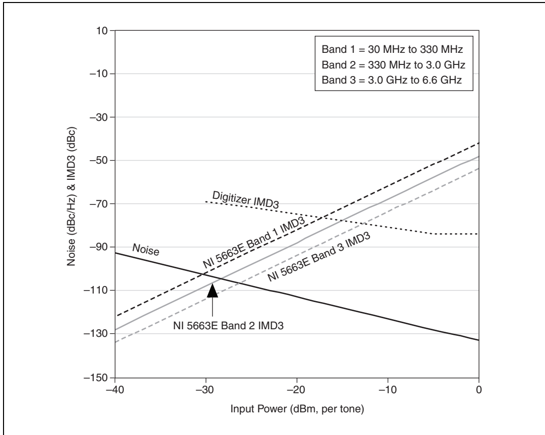
Figure 4. NI 5663E Vector Signal Analyzer Nominal Dynamic Range, 0 dBm Reference Level
