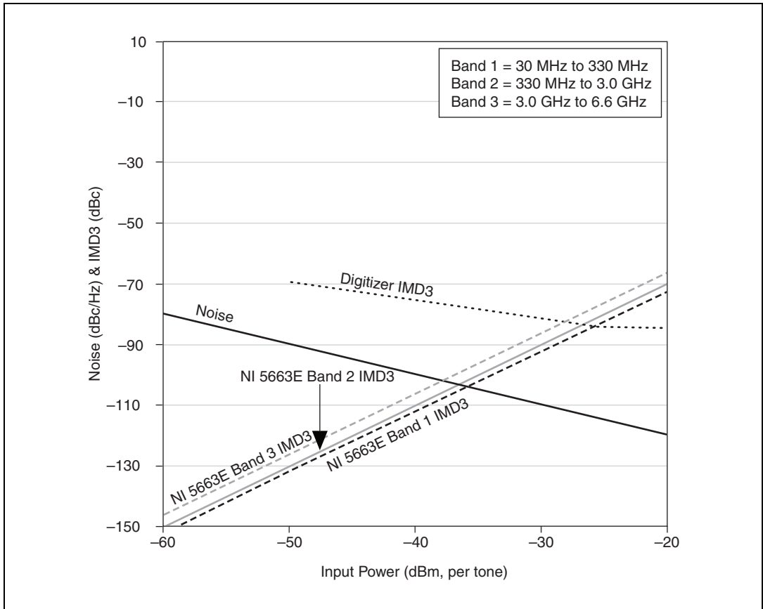
Figure 5. NI 5663E Vector Signal Analyzer Nominal Dynamic Range, -20 dBm Reference Level
