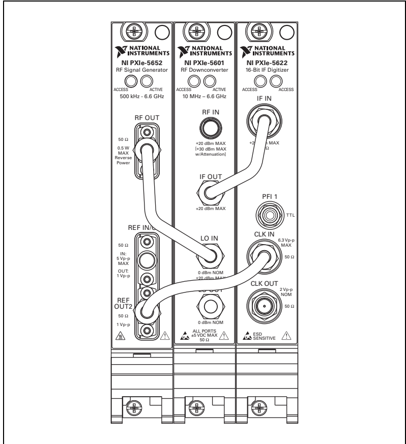
Figure 7. NI 5663E Front Panels
